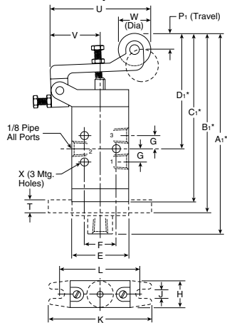
Roller Operated
