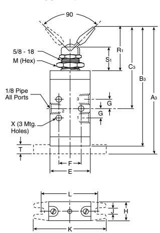
Toggle Operated
